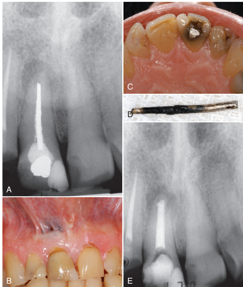
Fig. 9.22 Silver cones have been advocated for ease of placement and length control. A , Radiograph of a maxillary right central incisor obturated with a silver cone. B , Tissue discoloration indicating corrosion and leakage. C , Lingual view indicates coronal leakage. D , Corroded silver cone removed from the tooth. E , Posttreatment radiograph of the tooth.
